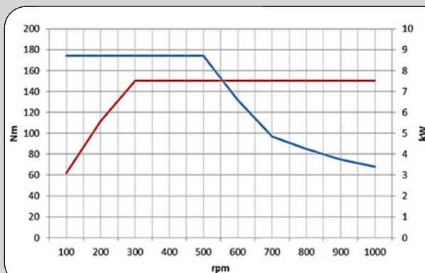
SPINDLE DIAGRAM STEP 1
