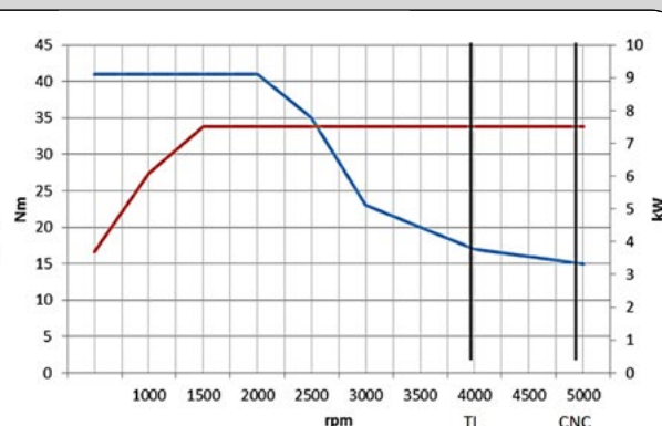
SPINDLE DIAGRAM STEP 2
